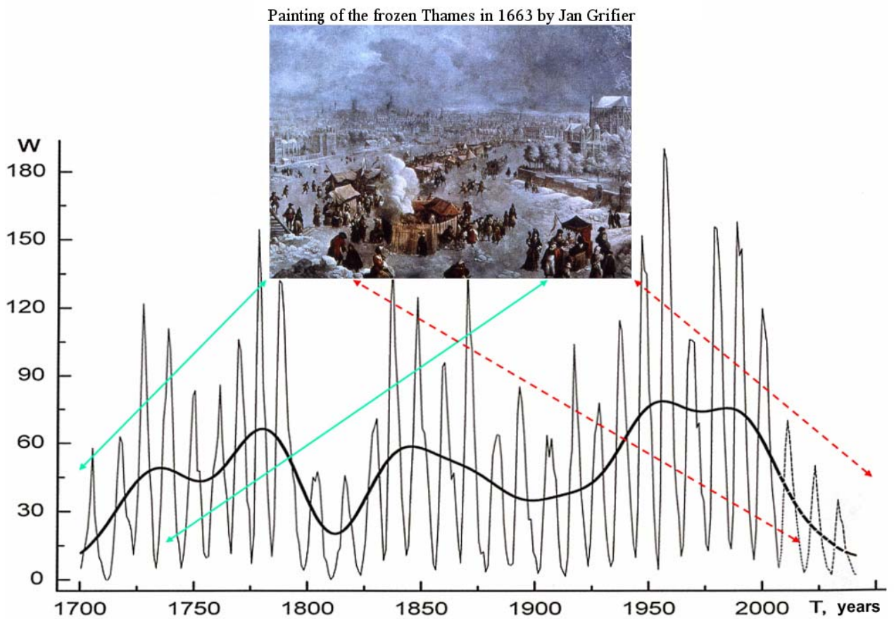
Fig. 5. Observed variations in the 11-year sunspot activity (continuous thin line) and the biccennial activity of the Sun (continuous heavy line) 1700-2008, and our forecast of variations in these values for the period of 2009-2042 (dotted lines).
